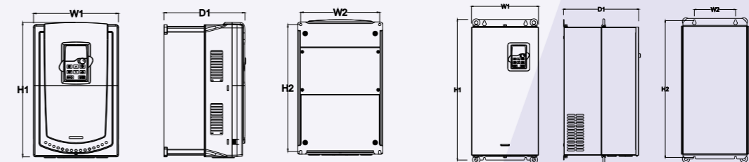
Wall installation of 220V 37~55kW VFDs Wall installation of 460V 37~110kW VFDs
