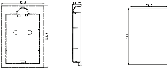
Pallet (SY8600-DP03)
